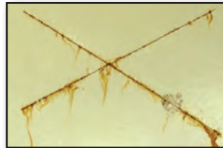
Common cold rolled sheet steel after a 336 hour salt spray test.
