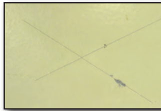
Galvanite™ cold rolled sheet steel with our powder coat finish after a 336 hour salt spray test.
